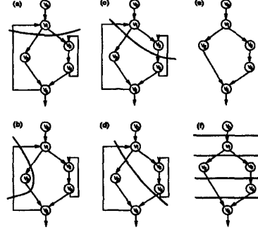
Figure 4: (a-d) Different logical cuts for an example NFG; (e) The acyclic NFG (ANFG); (f) Different cut points (levels).
