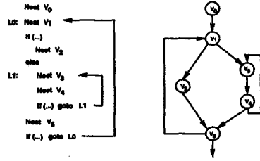
Figure 1: Left: a program fragment; Right: the Nest Flow Graph (NFG).
